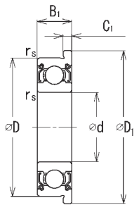
Shielded: ZZ
