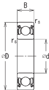
Shielded: ZZ
