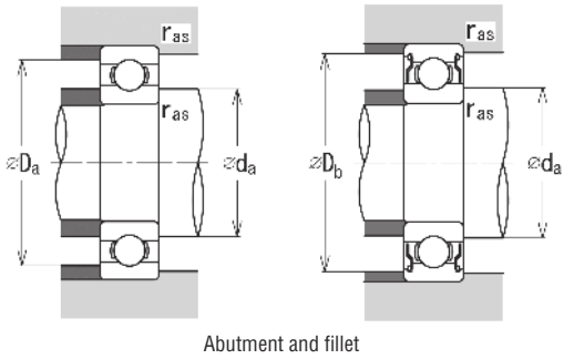
Abutment and fillet
