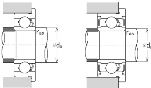
Abutment and fillet
