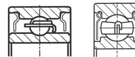
Root shield
